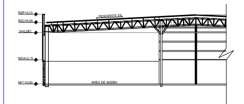
BUILDING SECTION
