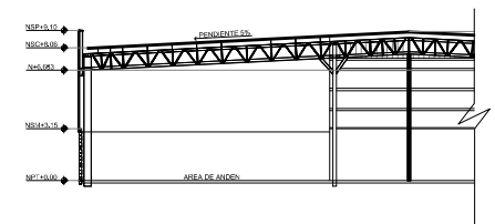
BUILDING SECTION
