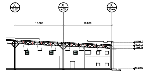
BUILDING SECTION
